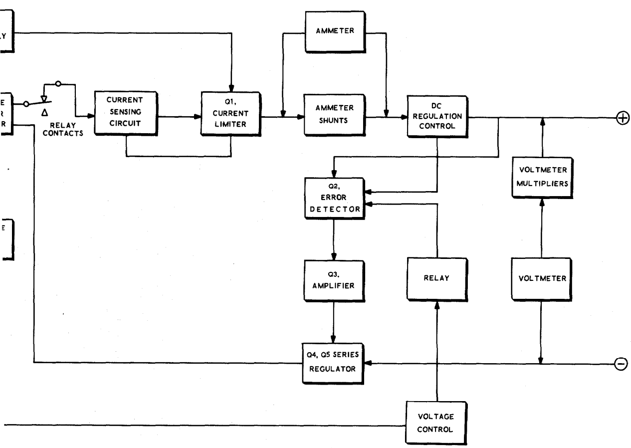
BLOCK DIAGRAM
